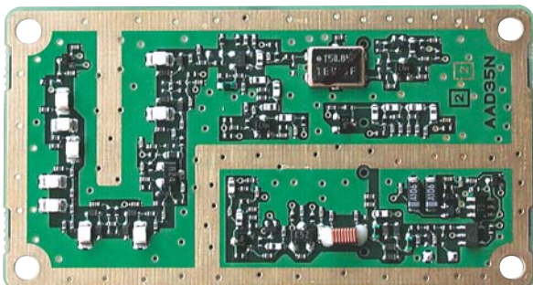
Multi Band Receiver Unit: SRX-1 for UHF, SRX-2 for VHF
